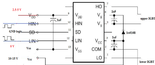
Fig 6: Driver Circuit operation
