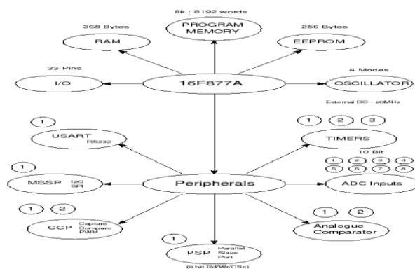
Fig 2: Micro-controller Peripherals
