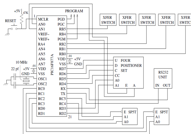
Fig 3: Microcontroller PIC16F877A
