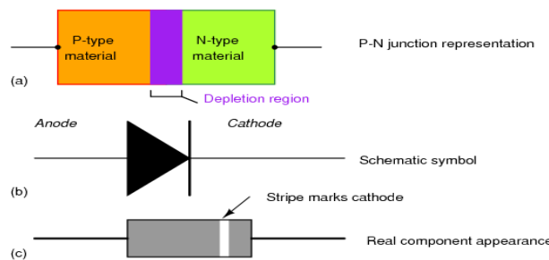
Fig 11: Diode
